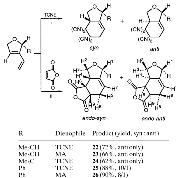
Scheme 3 TCNE = tetracyanoethylene, MA = maleic anhydride; i, benzene, 2 h, 25 °C, TCNE (1.2 equiv.); ii, MeCN, 80 °C, 10 h, MA (2.0 equiv.)
