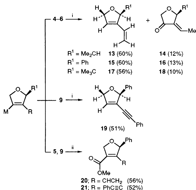
Scheme 2 M = CpW(CO) 3 ; i, Me 3 NO·H 2 O (5 equiv.), CH 2 Cl 2 (23 °C, 5 h); ii, CO (1 atm), (NH 4 ) 2 Ce(NO 3 ) 6 (3.0 equiv.), MeOH-CH 2 Cl 2 (1:1, -78 °C, 4 h)
